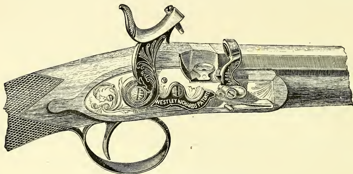
The Westley Richards Detonating Gun.
